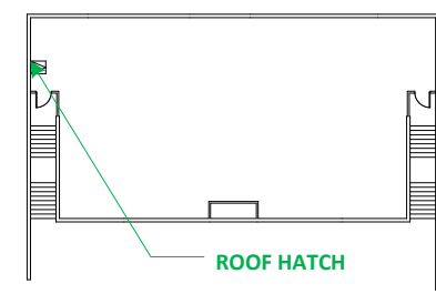
GYM MEZZANINE PLAN
